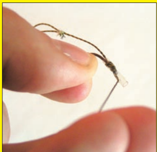
9. Pull the eye of the hook into the shrink tube
